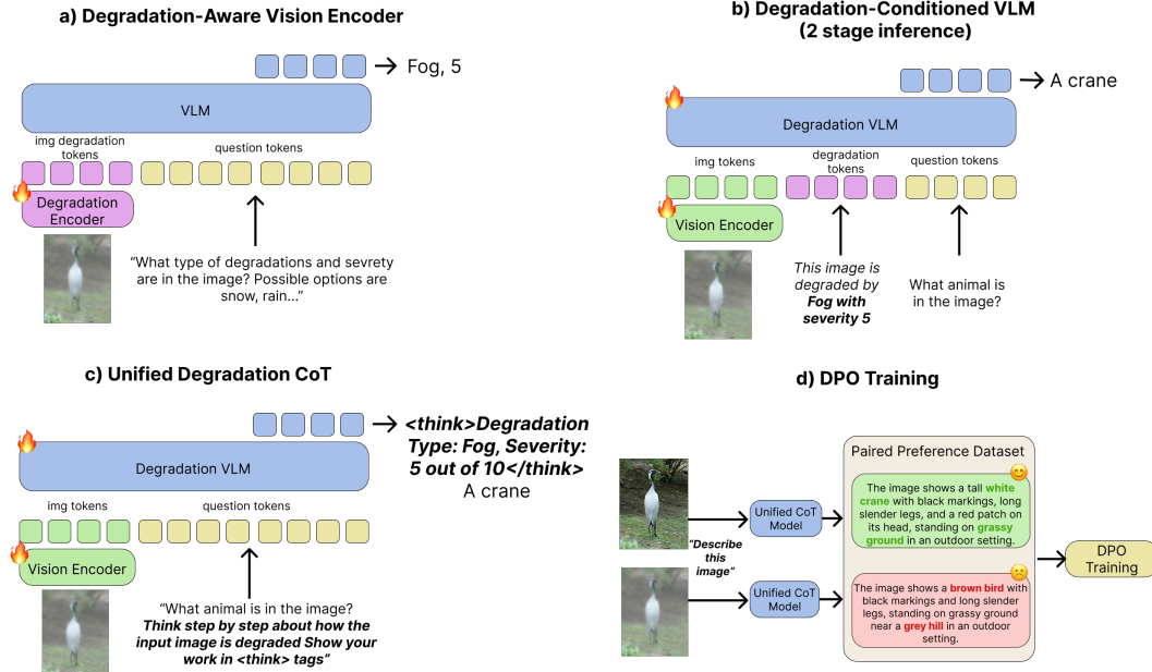
Figure 2: Multistep training to a unified degradation-robust VLM. We transform a pre-trained VLM into a single-pass degradation-robust reasoning pipeline through sequential fine-tuning. (a) Degradation encoder: we fine-tune the vision encoder to predict degradation type and severity from the degraded image. (b) Degradation-conditioned VLM: we fine-tune the language model to perform captioning/QA conditioned on the explicit degradation tokens, yielding robustness but requiring two-step inference (predict degradation, then answer). (c) Unified degradation CoT: we unify the pipeline into one forward pass by training the model to first verbalize degradation type/severity within <think> tags and then produce the final answer, using the generated reasoning trace as implicit conditioning.
